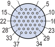
Insert Arrangement 12-37, 13-37, 15-37 37 #23 Contacts .022 (0.56) Max. Dia. Tail
