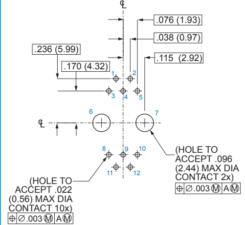
Socket Connector
