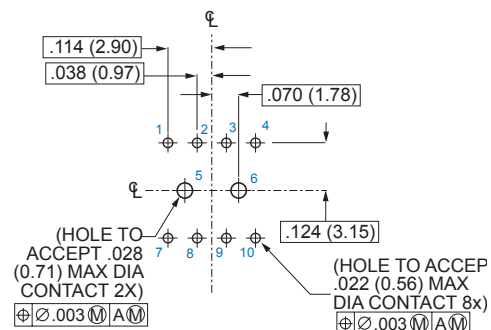
Socket Connector
