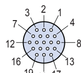
Insert Arrangement 9-19, 11-19 19 #23 Contacts .022 (0.56) Max. Dia. Tail
