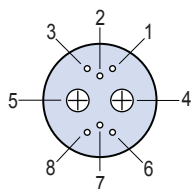
Insert Arrangement 12-200, 13-200, 15-200 2 #12 Contacts 6 #23 Contacts
