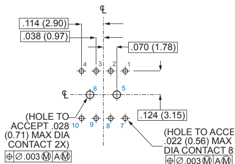
Pin Connector
