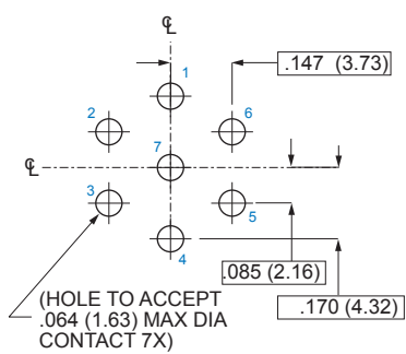
Socket Connector
