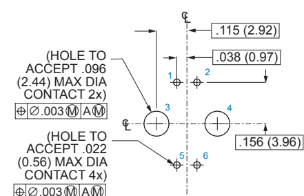
Socket Connector
