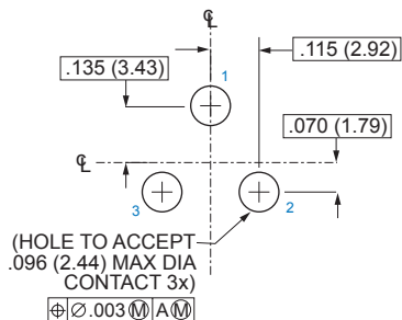
Pin Connector
