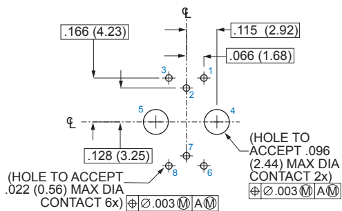
Pin Connector
