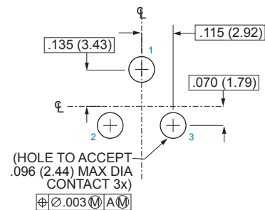
Socket Connector
