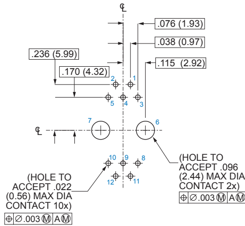
Pin Connector
