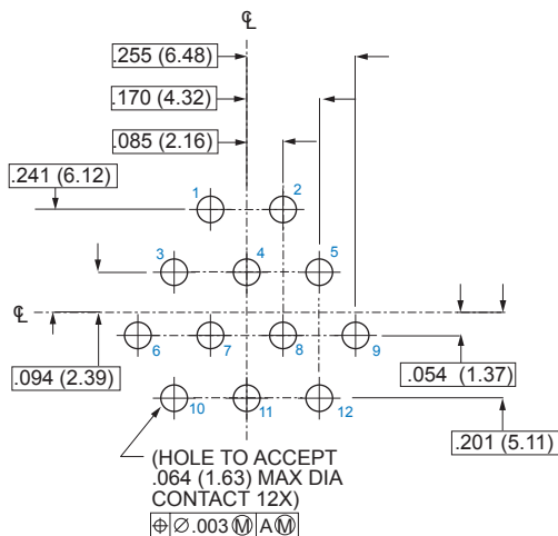
Socket Connector
