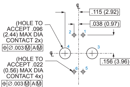
Pin Connector
