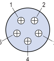
Insert Arrangement 14-5, 16-5, 18-5 5 #12 Contacts
