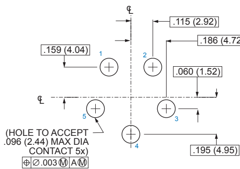
Pin Connector
