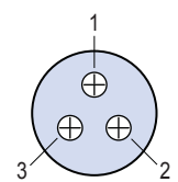
Insert Arrangement 12-3, 13-3, 15-3 3 #12 Contacts
