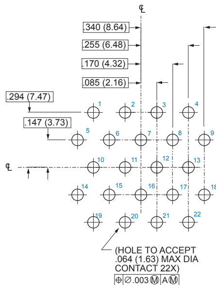
Socket Connector
