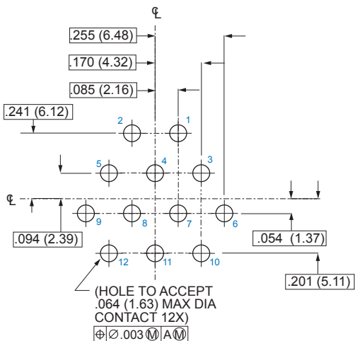
Pin Connector
