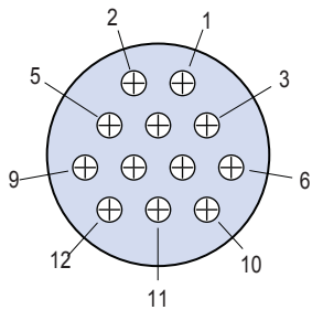
Insert Arrangement 21-12, 23-12 12 #12 Contacts
