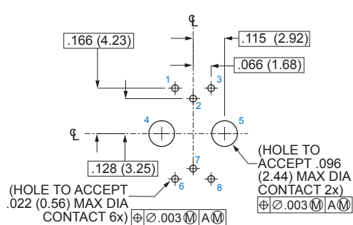
Socket Connector
