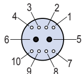
Insert Arrangement 9-201, 11-201 2 #20 Contacts 8 #23 Contacts
