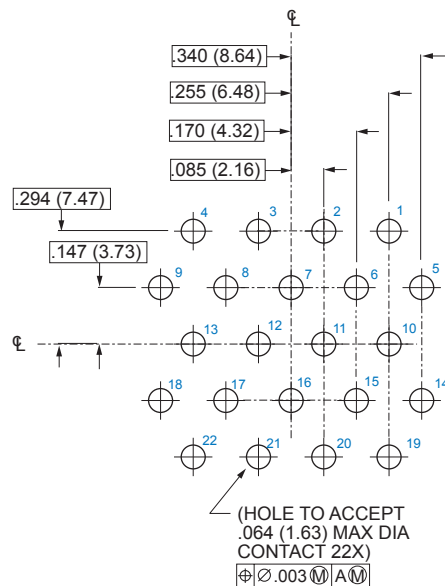
Pin Connector
