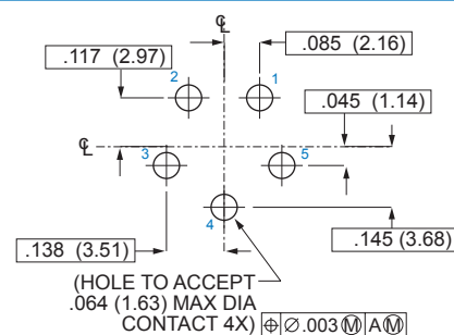
Socket Connector
