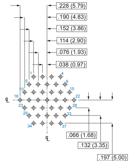
Socket Connector
