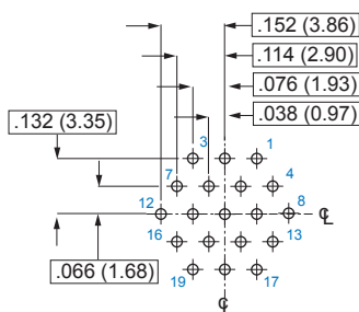
Pin Connector
