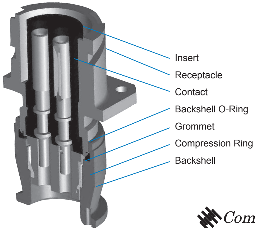
-00 Wall Mount Receptacle
